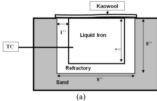
Figure 5. These mold designs were used in Experiment 1: View (a) schematic design of the mold; (cont'd.)
