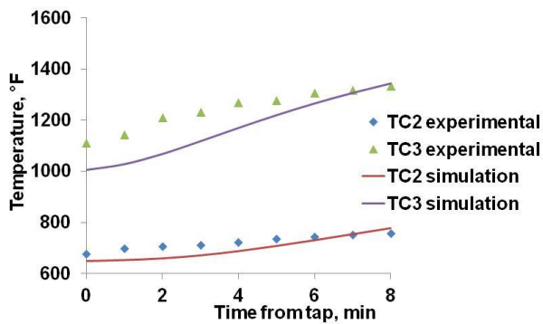
Figure 12. Graph shows the comparison between experimental and CFD simulated lining temperature for 100 lb (45 kg) ladle lined with the novel refractory (silica + 30 vol. % cenospheres). e novel refractory (silica + 30 vol. % cenospheres). [3]
