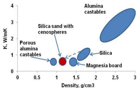
Figure 1. Room temperature thermal conductivity versus density of different refractory materials is shown. [3] (Artwork courtesy of ST Foundry, Inc.)
